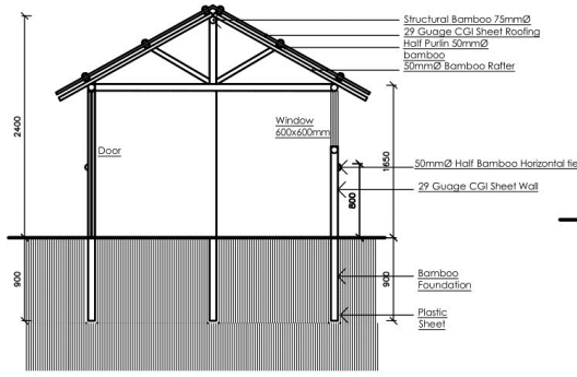
Cross-Section
