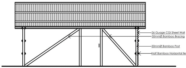
Typical Bracing (long wall)
