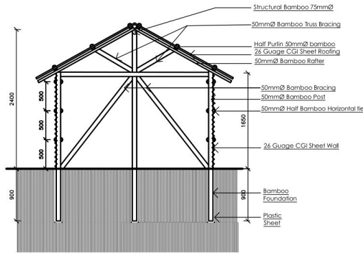
Typical Bracing (side wall)
